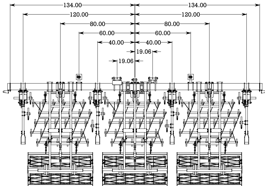
3 ROW 80" LAYOUT
