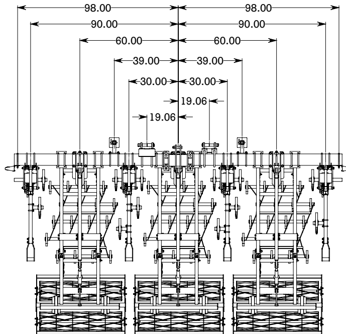
3 ROW 60" LAYOUT
