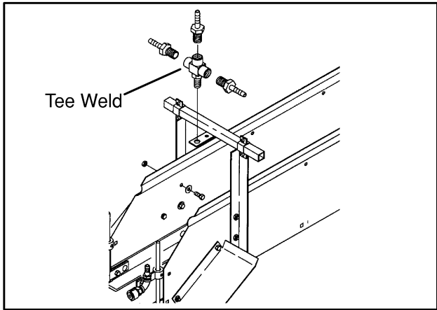
Figure 174. Top Spray Bracket
