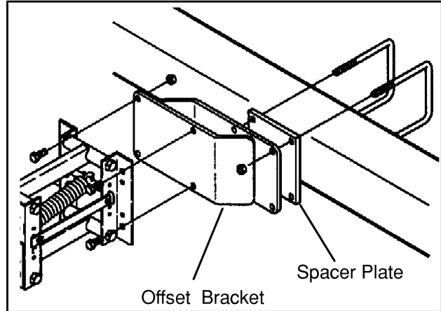
Figure 176. Mounting Offset Bracket
