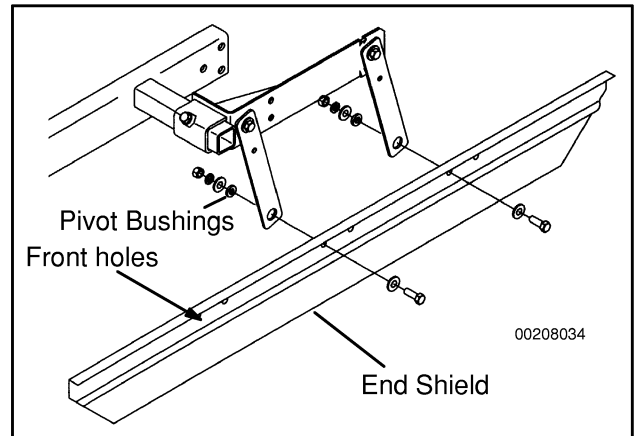
Figure 123. Fastening End Shields
