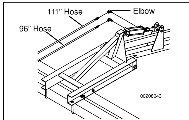
Figure 167. Mounting Hydraulics
