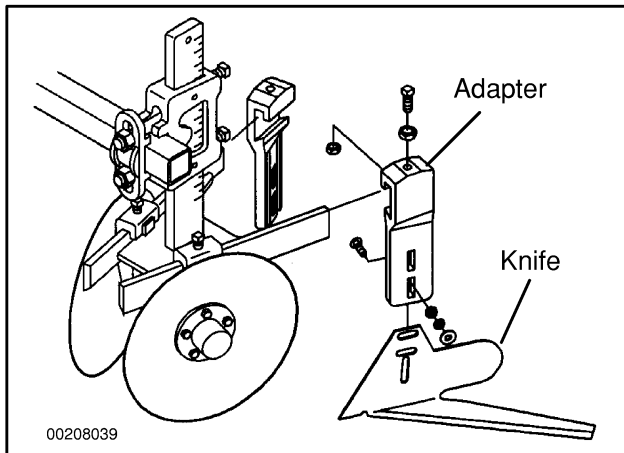
Figure 145. Dual Knife
