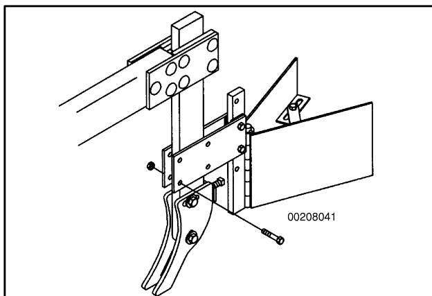
Figure 156. Fastening to Shank
