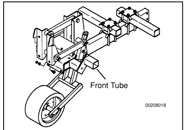
Figure 58. Offset Front Tubes
