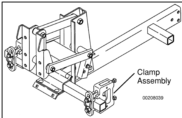
Figure 142. Fastening Clamp
