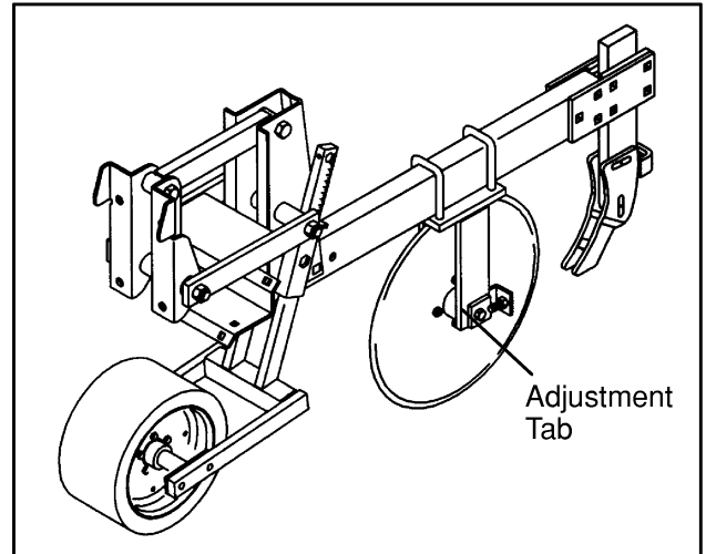
Figure 19. Coulters Disc (2065)
