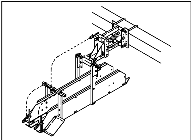
Figure 175. Hoses
