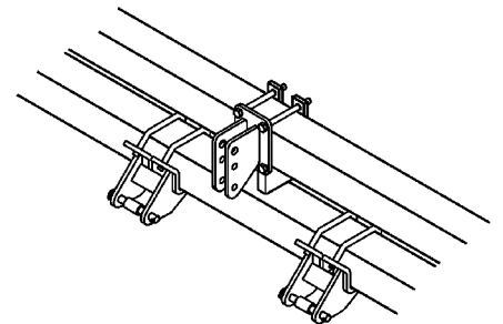
E. 3 piece heavy duty hitch for top reinforced 7" x 7" beams. Recommended on all TRF tool bars.
