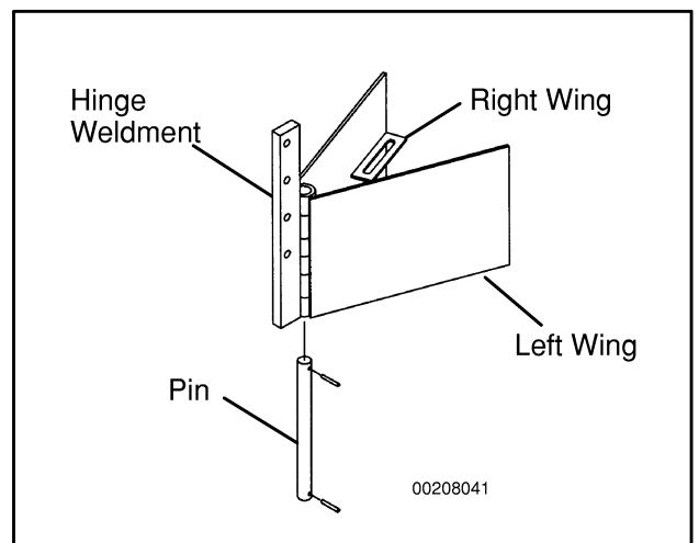
Figure 153. Assembling Hiller
