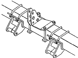
C. 4 piece hitch for 7" x 7" beams. Recommended on 8 row and smaller units.
