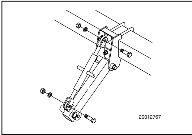
Figure 93. Attaching Screwjack
