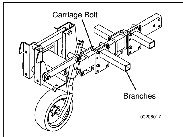
Figure 54. Tine Tree
