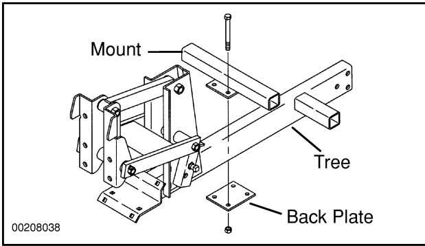
Figure 136. Fastening Mount
