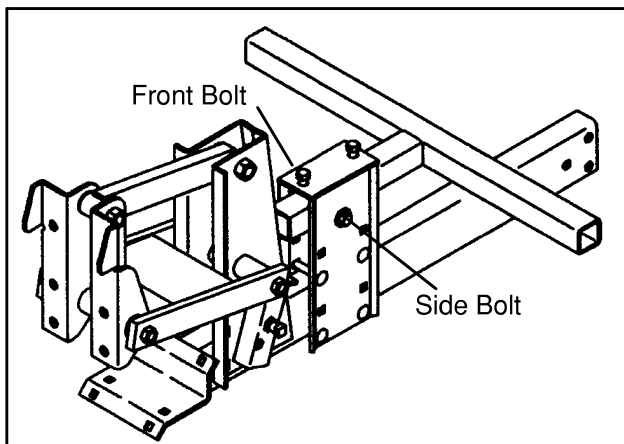
Figure 22. Slide Mount Tunnel Shields
