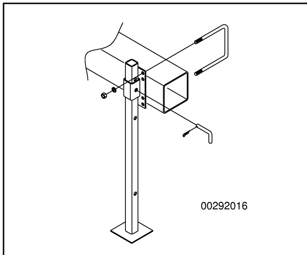
Figure 102. Mounting Parking Stand
