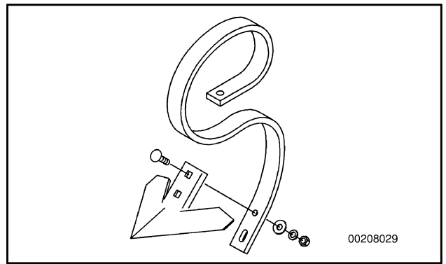
Figure 87. Penetrator Tine
