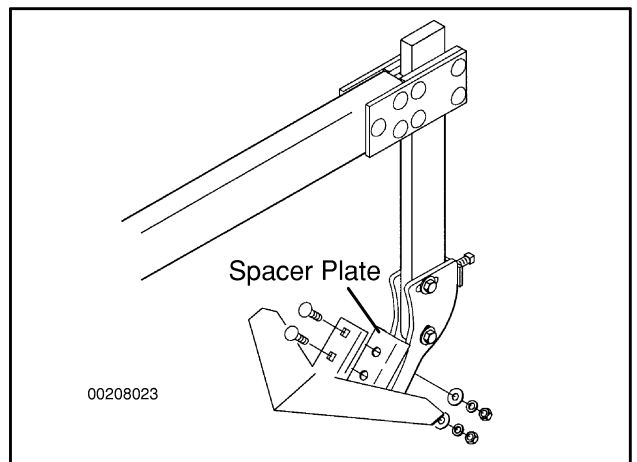
Figure 89. Rear Shank
