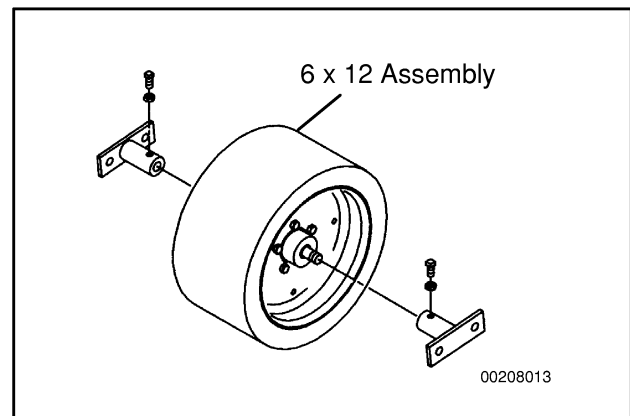
Figure 44. Bushing Plates
