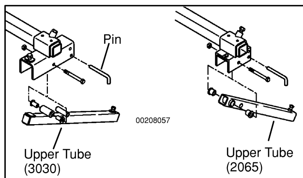
Figure 130. Fastening Tubes
