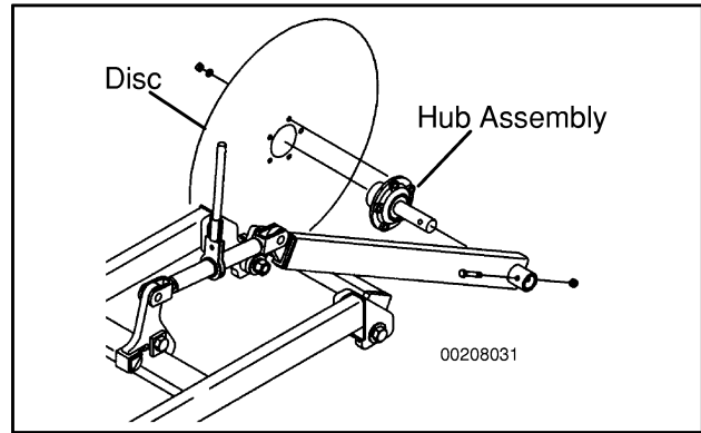
Figure 108. Mounting Disc
