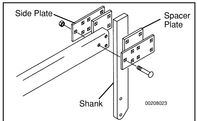
Figure 68. Mounting Shank
