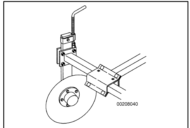
Figure 152. Mounting Crank Assembly
