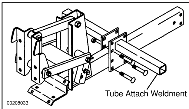
Figure 126. Branch Mounted
