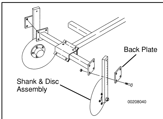
Figure 150. Mounting Discs
