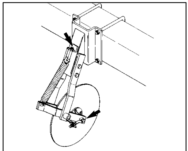
Figure 20. Front Stabilizer Coulters
