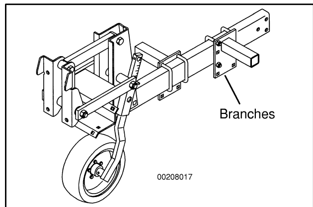
Figure 53. Tine Tree
