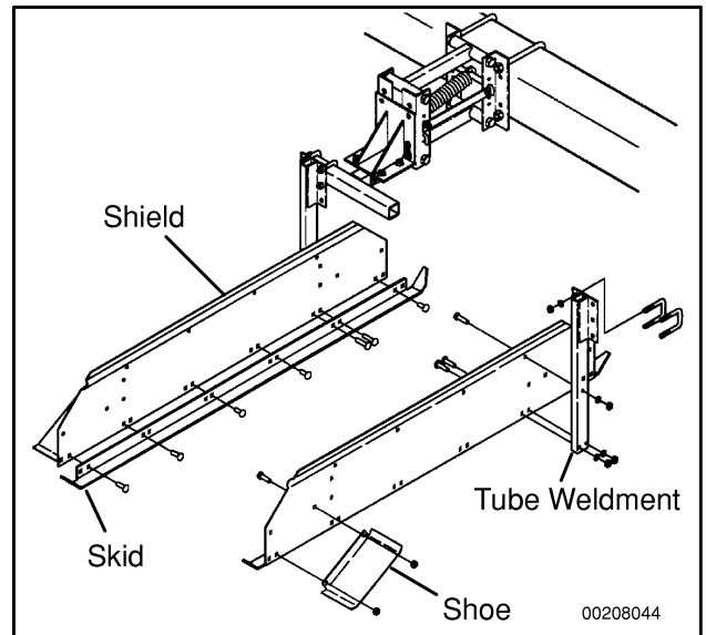
Figure 171. Mounting Shields
