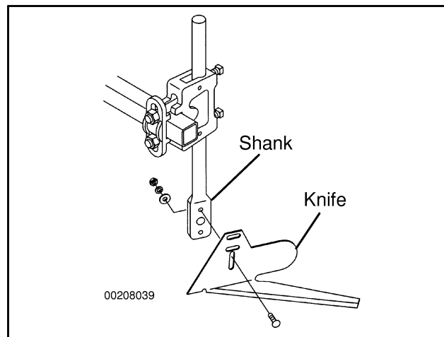
Figure 148. Mounting Knives
