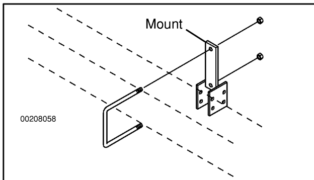
Figure 125. Toolbar Mounted
