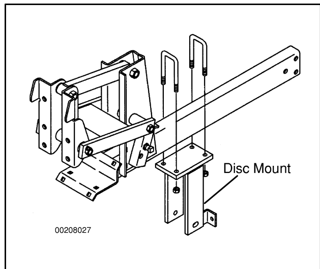
Figure 73. Disc Mount
