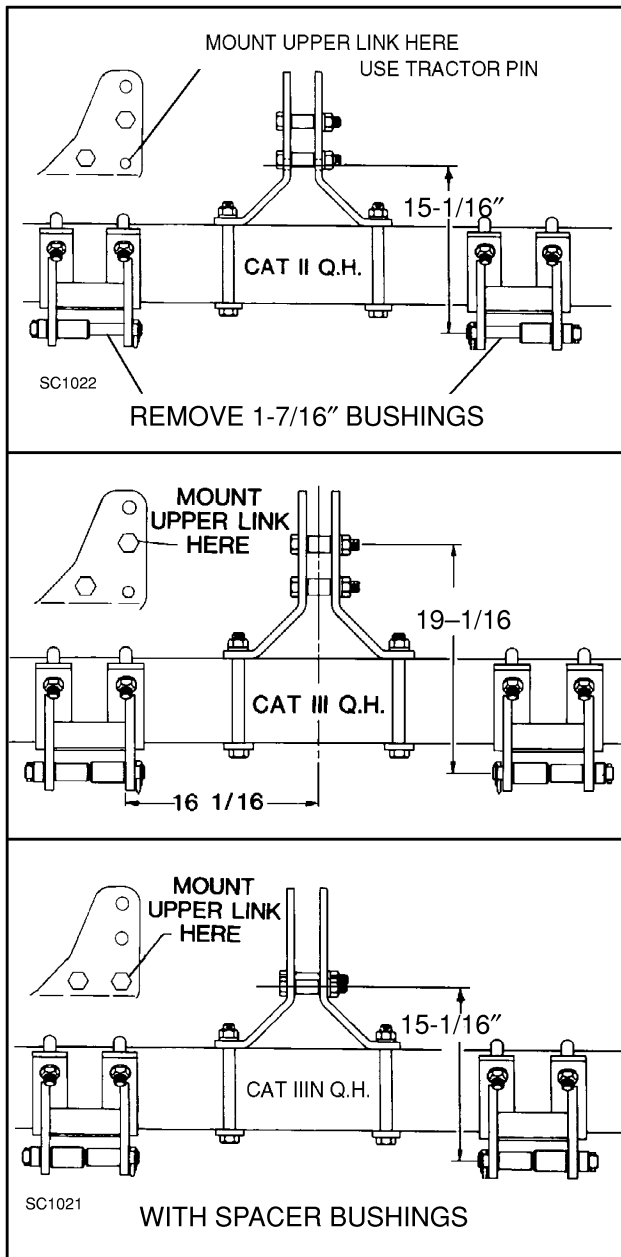
Figure 32. Quick Hitches
