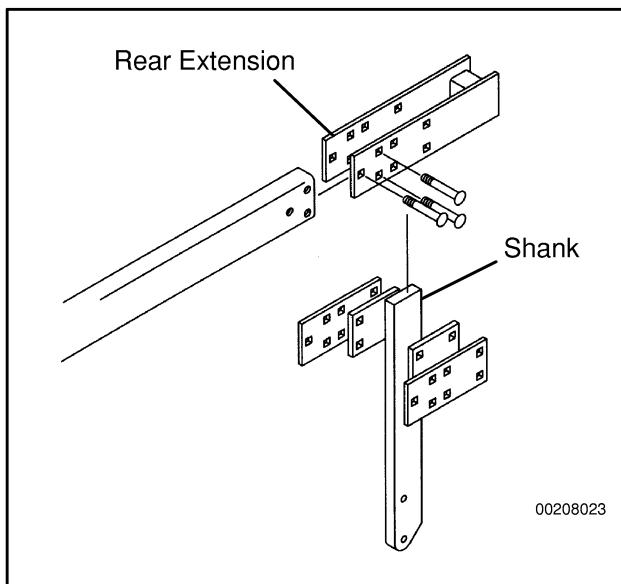
Figure 66. Rear Extension - Model 2065
