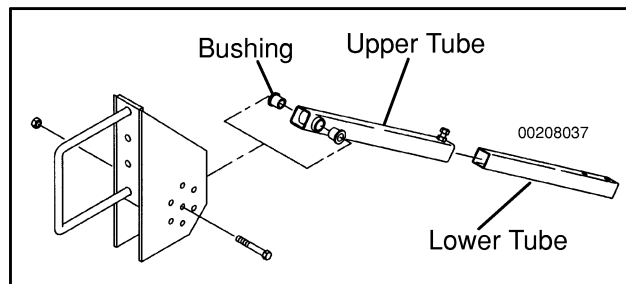
Figure 129. Fastening Tubes
