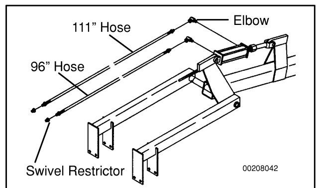
Figure 163. Mounting Hydraulics
