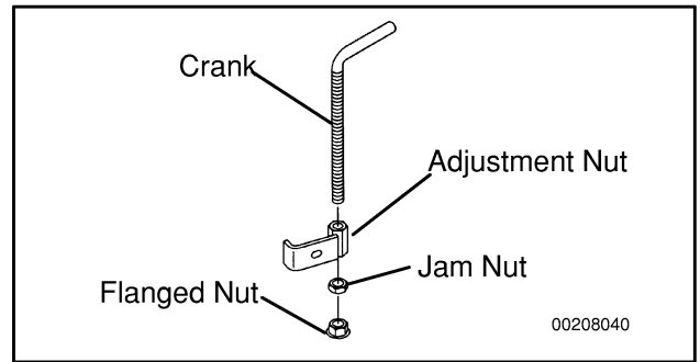
Figure 151. Disc Crank
