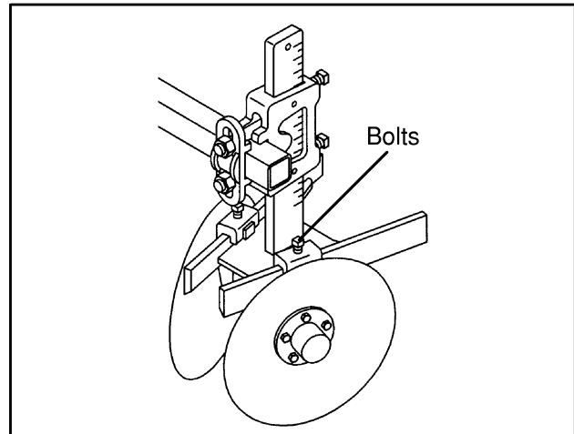
Figure 23. Dual Discs
