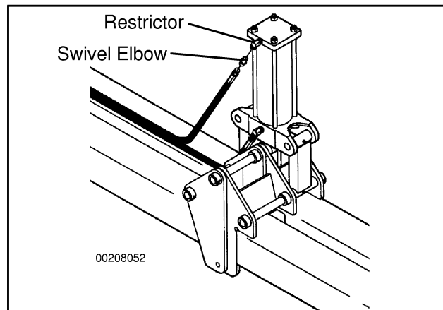
Figure 36. Fittings
