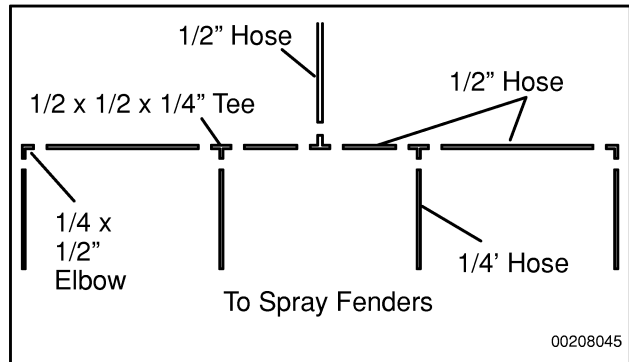
Figure 177. Plumbing Toolbar
