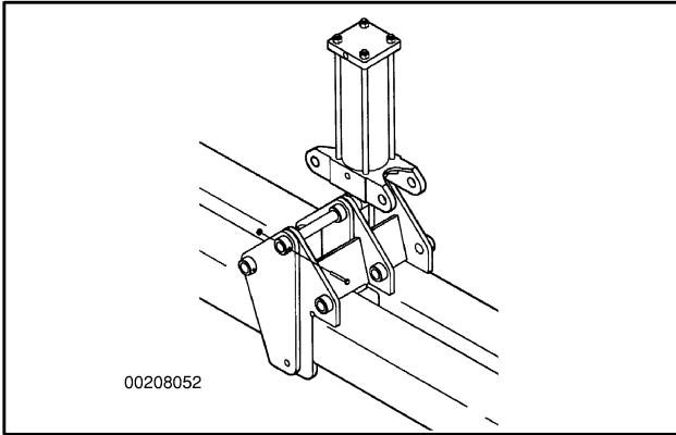
Figure 34. Mounting Wings
