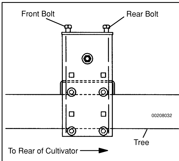
Figure 112. Adjusting
