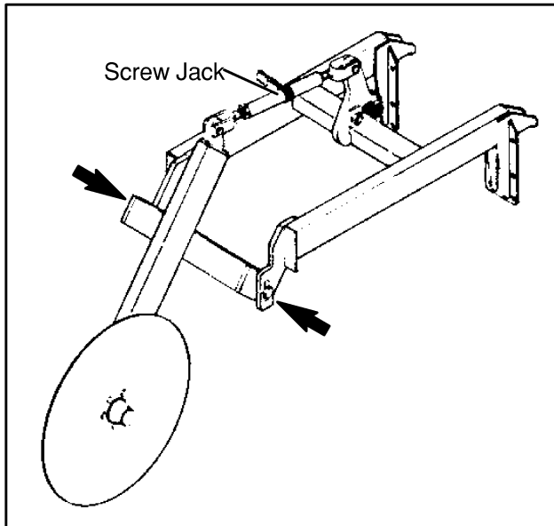
Figure 21. Rear Stabilizer
