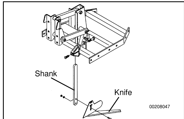
Figure 185. Mounting Knives
