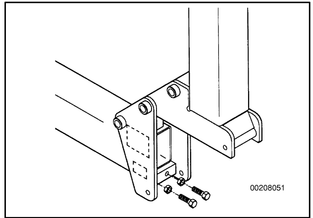
Figure 39. Leveling Wings
