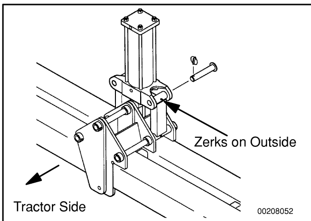
Figure 35. Cylinder Linkage Bars
