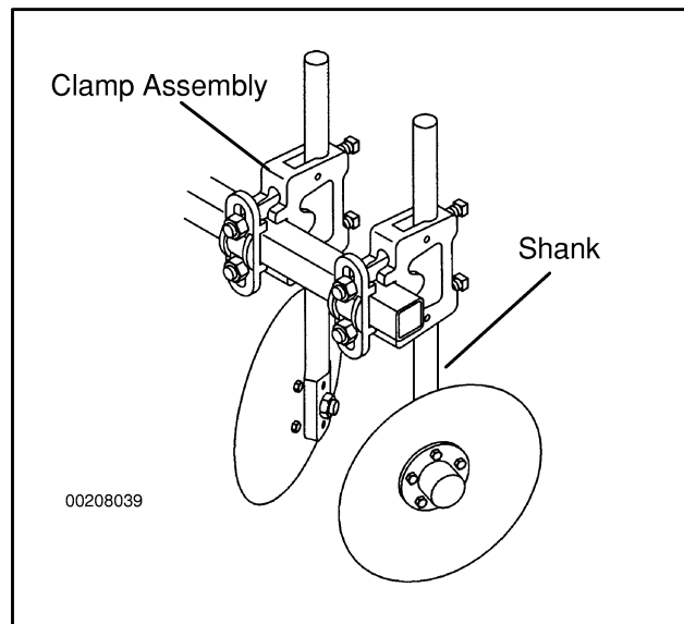
Figure 147. Mounting Discs
